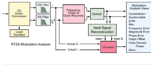
Figure 2-18: RSA modulation analysis block diagram.
