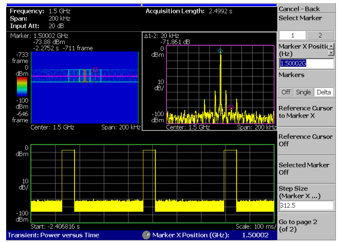
Figure 1-14: Multi-domain view showing spectrogram, power vs. frequency, and power vs. time.
