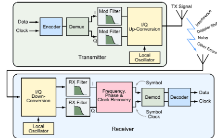
Figure 2-17: Typical digital communications system.
