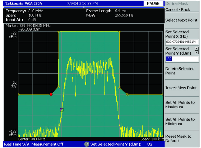
Figure 2-9: Frequency mask definition.
