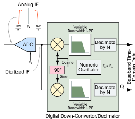
Figure 2-2: Digital down-converter block diagram.
