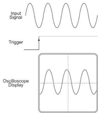
Figure 2-6: Traditional oscilloscope triggering.
