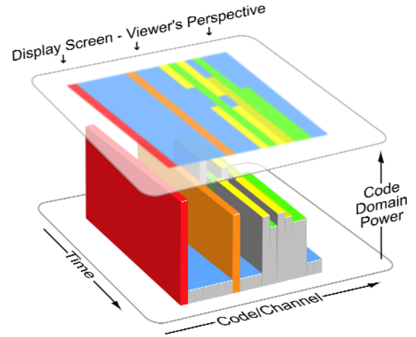
Figure 3-19: Illustration of the codogram display.
