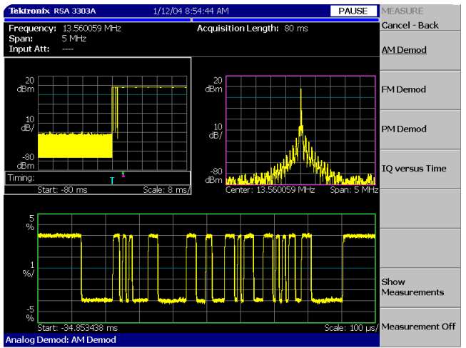
Figure 3-11: AM demod analysis of a pulsed signal using amplitude shift keying to encode data.
