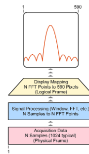
Figure 4-3: Standard SA mode data mapping for spans less than the real-time bandwidth.
