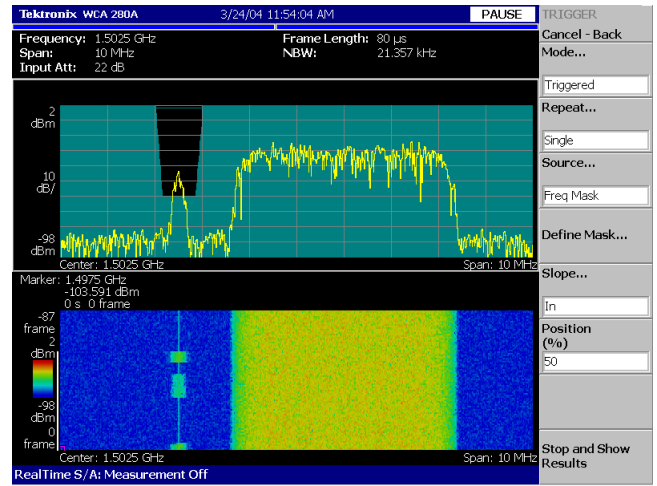
Figure 1-8: Using the frequency mask to trigger on a low level burst in the presence of a large signal.
