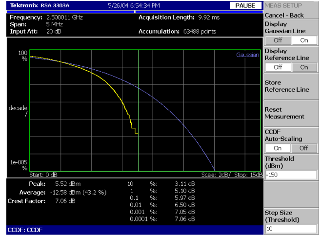
Figure 3-9: CCDF measurement.
