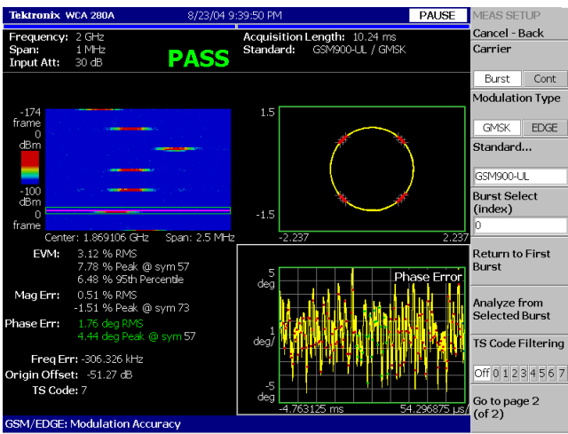
Figure 3-18: Spectrogram, constellation, EVM, and phase error vs. time of frequency hopping GSM signal.
