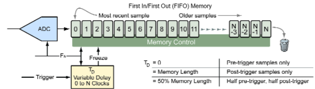
Figure 2-7: Triggering in digital acquisition systems.
