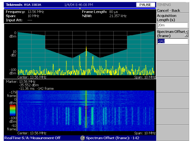
Figure 1-9: Using the frequency mask to trigger on a specific signal in a crowded spectral environment.
