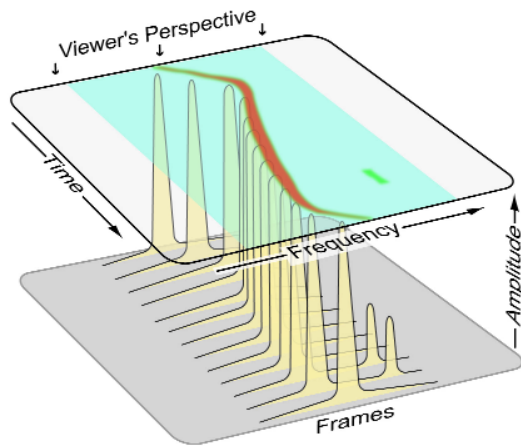
Figure 1-10: Spectrogram display.
